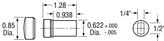
HOLDER ASSEMBLY • P/N 1092006 Material: Brass, tin plated (plastic cap included)
