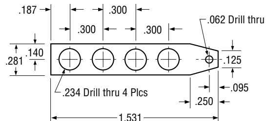
BUSS ASSEMBLY • P/N 1070011-9
