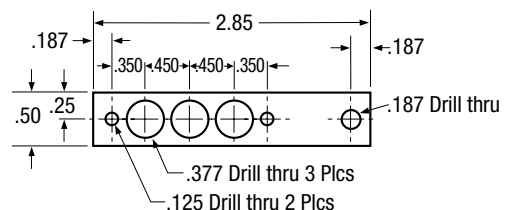
FLAT BUSS ASSEMBLY • P/N 1913003-7
